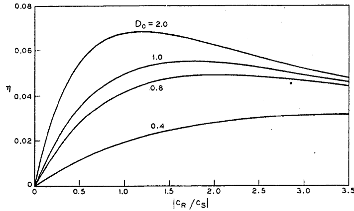
Fig. 18—Reflection holograms—the efficiency of an absorption grating as a function of slant for \alpha_1 = \alpha ( D_1 = D_0 ). c = c_R/c_S is the slant factor.
