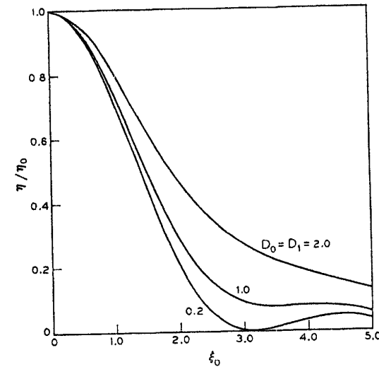
Fig. 17—Reflection holograms—the angular and wavelength sensitivity of an absorption grating for \alpha_1 = \alpha ( D_1 = D_0 ) and values of D_1 = 2\nu = D_0 = 0.2 ( \eta_0 = 0.007 ), D_1 = 1 ( \eta_0 = 0.05 ), and D_1 = 2 ( \eta_0 = 0.068 ).
