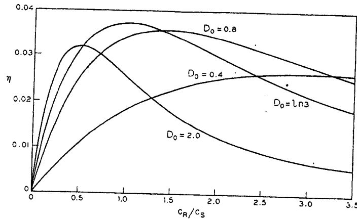
Fig. 11—Transmission holograms—the efficiency of an absorption grating as a function of slant for \alpha_1 = \alpha ( D_1 = D_0 ). c = c_R/c_S is the slant factor.
